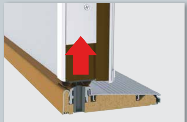
Flush Bolt and Floating Boot lift clear of the sill for damage-free operation.
